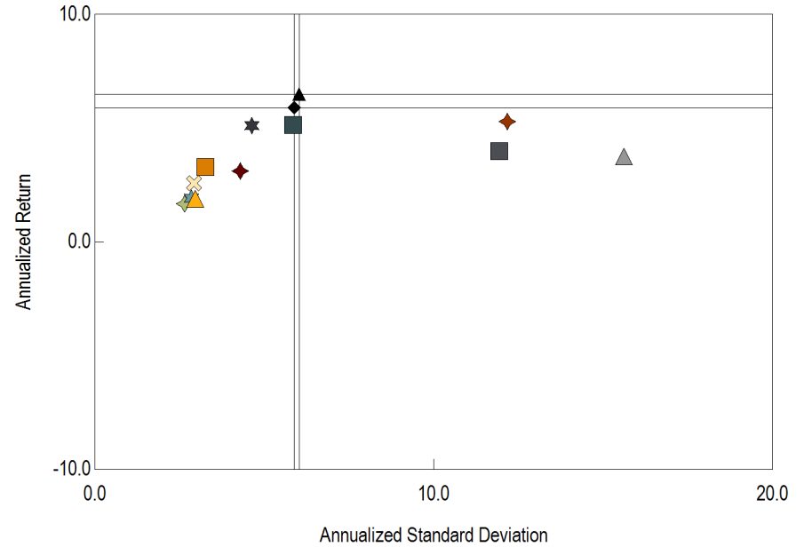
Annualized Return vs. Annualized Standard Deviation 3 Years Ending June 30, 2018
